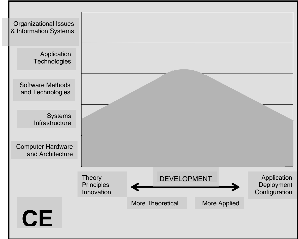
Figure 2.3. Computer Engineering
