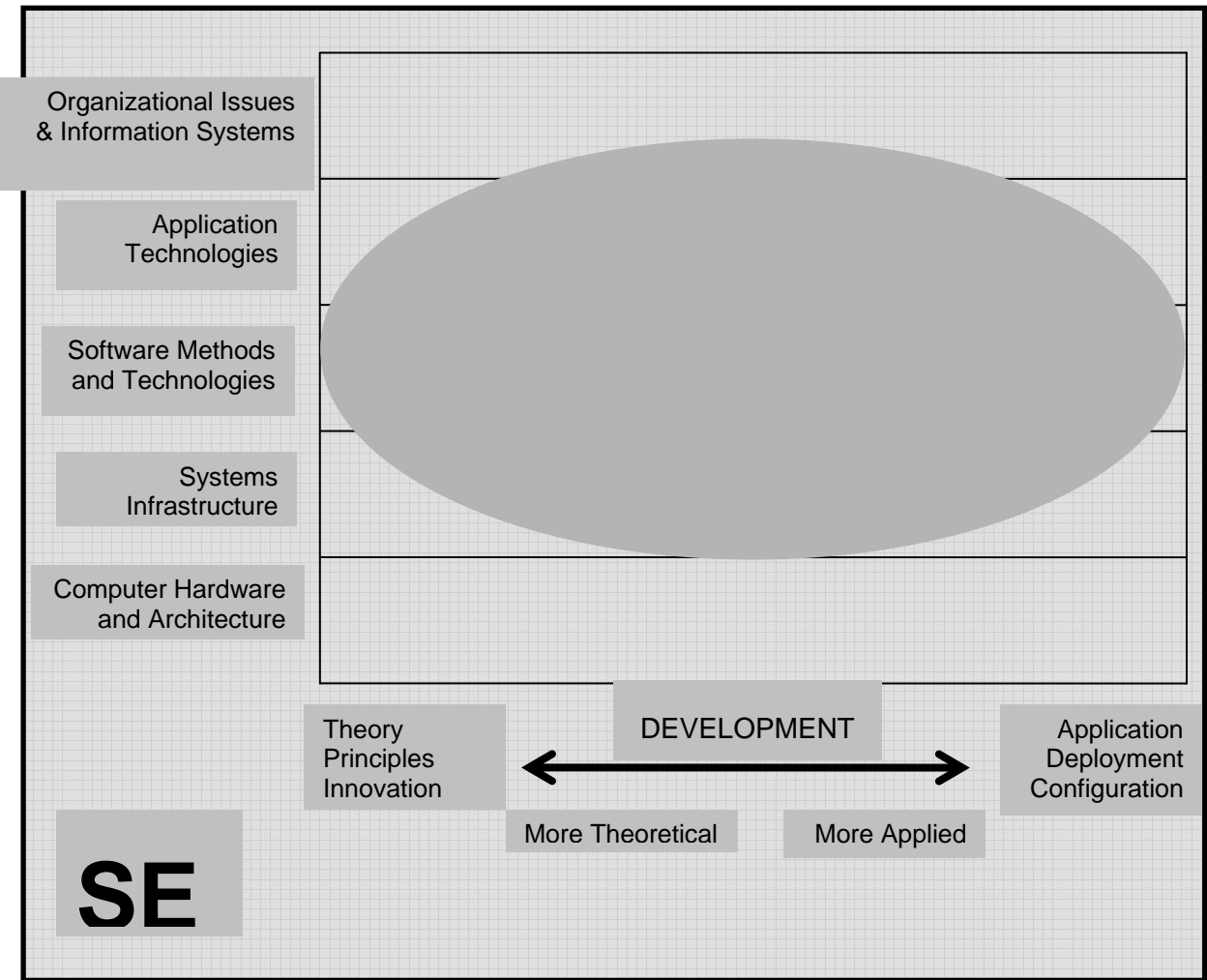
Figure 2.7. Software Engineering
