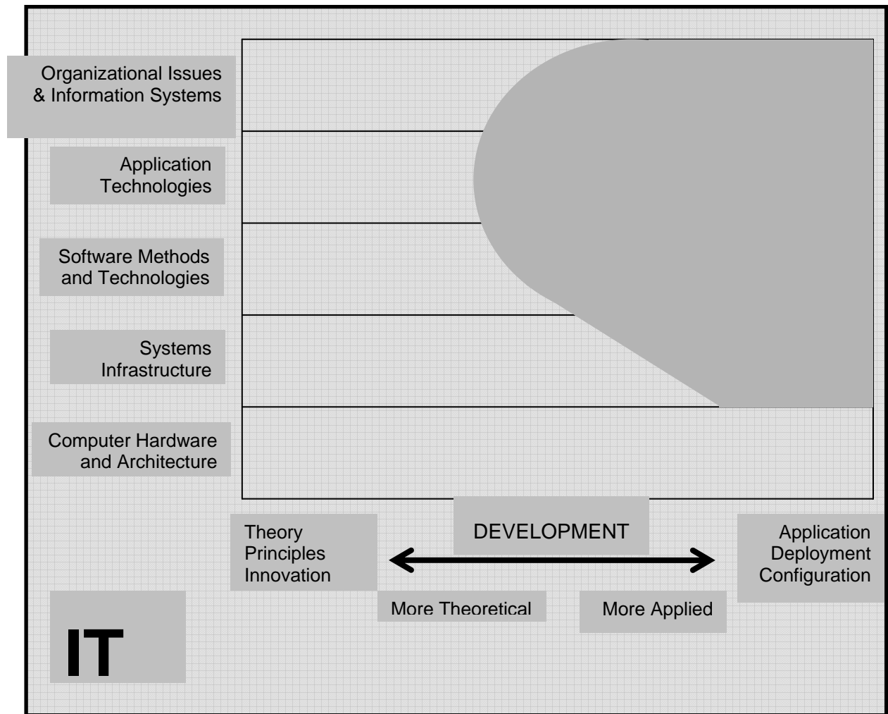
Figure 2.6. Information Technology
