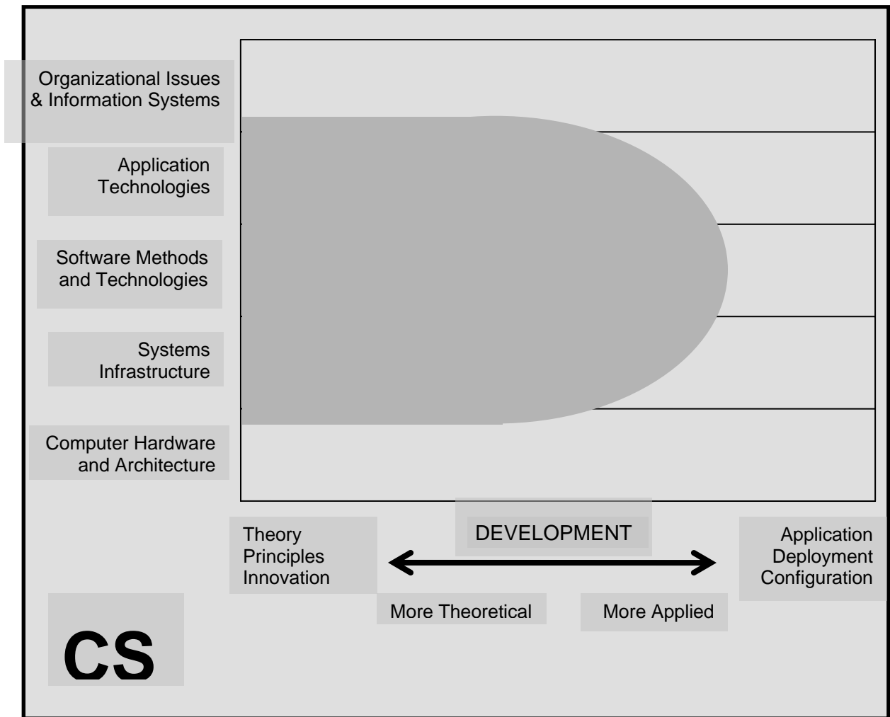
Figure 2.4. Computer Science
